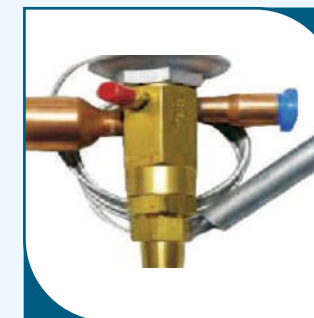
Expansion Valve
